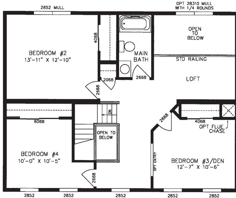
PLAN NO. PT5711 SECOND FLOOR 27'4" X 36'0"
